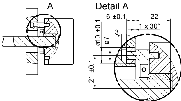
EAM580R, torque pin
