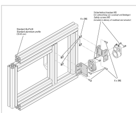
› Figure Sliding door
