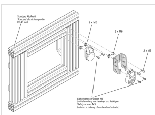
› Installation example mounting plate EMP Hinged door
