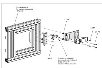
› Installation example mounting plate EMP Hinged door
