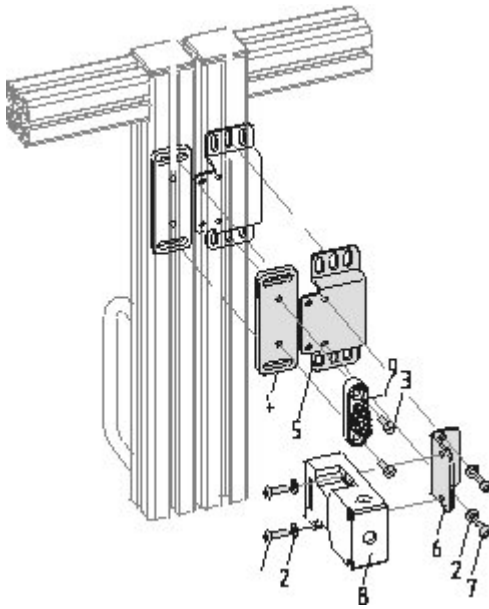
Product graph (exploded-view drawing)
