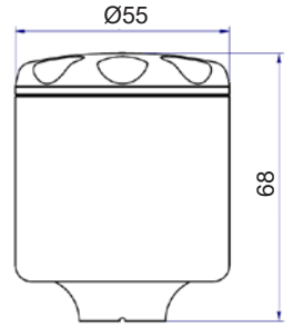
Ø55 mm housing
