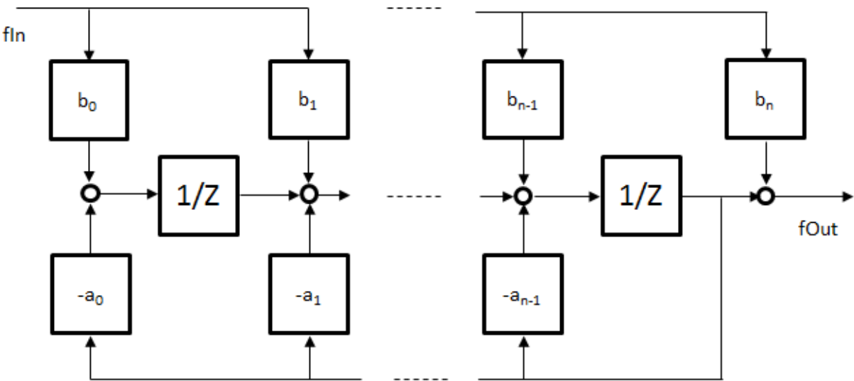
Fig. 1: FB_CTRL_Transferfunction_2_Signal
