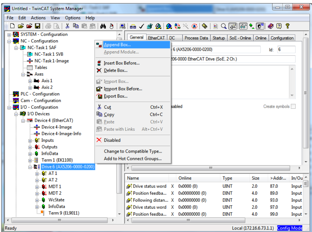
Fig. 4: Addition of an AX5805
