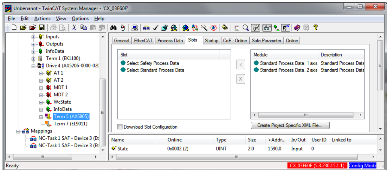
Fig. 6: Inserting the safety module into the AX5805
