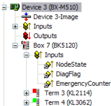
Fig. 58: NodeState, DiagFlag and EmergencyCounter
