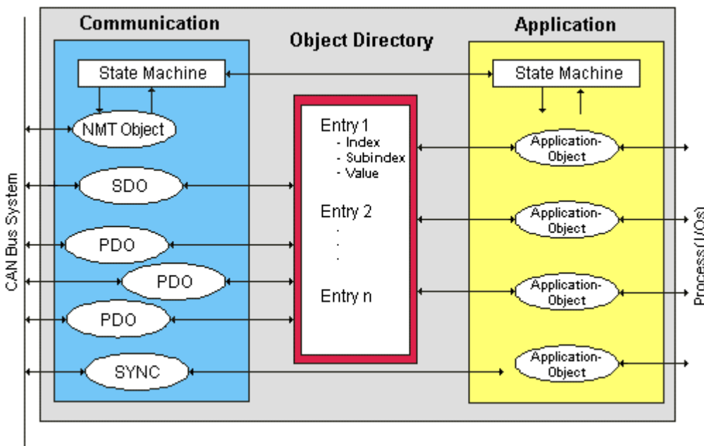
Fig. 127: CANopen Device Model
