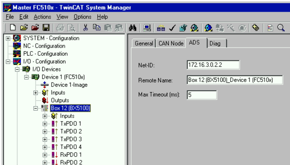
Fig. 123: Display of the BX5100 in the TwinCAT System Manager
