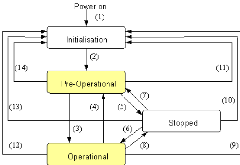
Fig. 128: CANopen bootup state diagram
