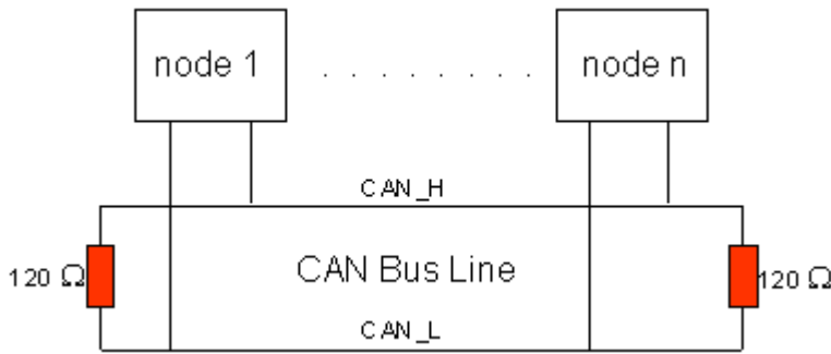
Fig. 17: Termination of the bus with a 120 Ohm termination resistor
