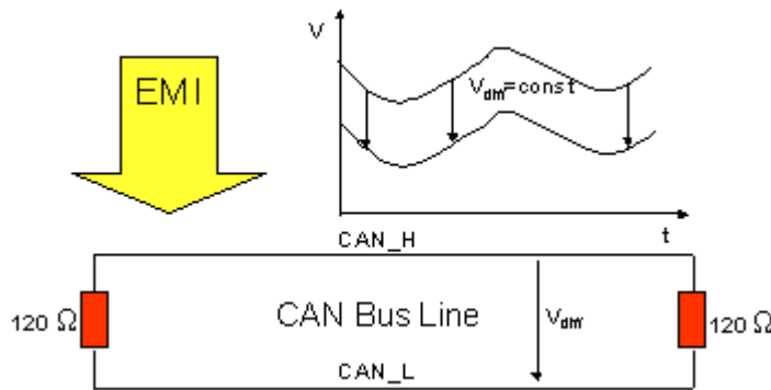
Fig. 18: Insensitivity to incoming interference
