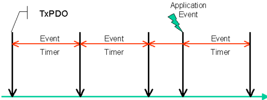
Fig. 136: Time representation of the event timer
