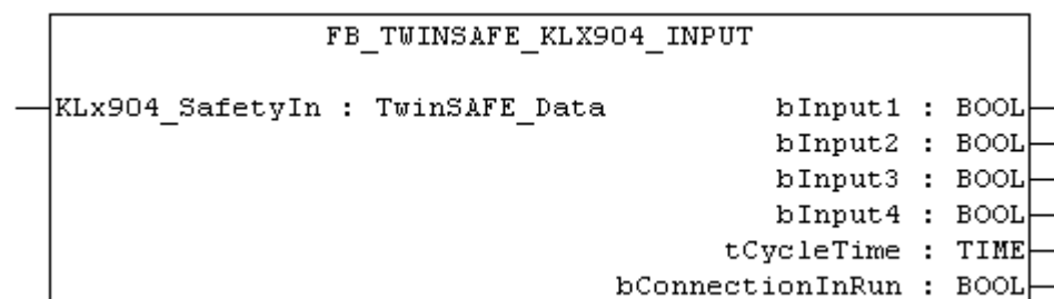
Fig. 110: Function block FB_TWINSAFE_KLX904_INPUT
