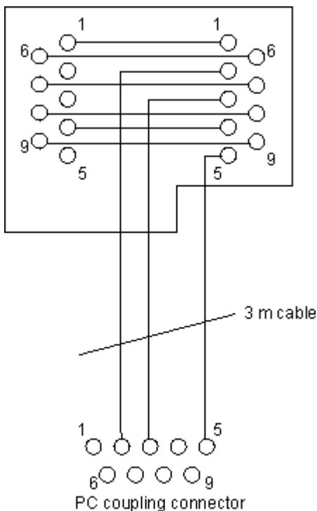
Fig. 14: Programming cable ZK1000-0030 - Pinning
