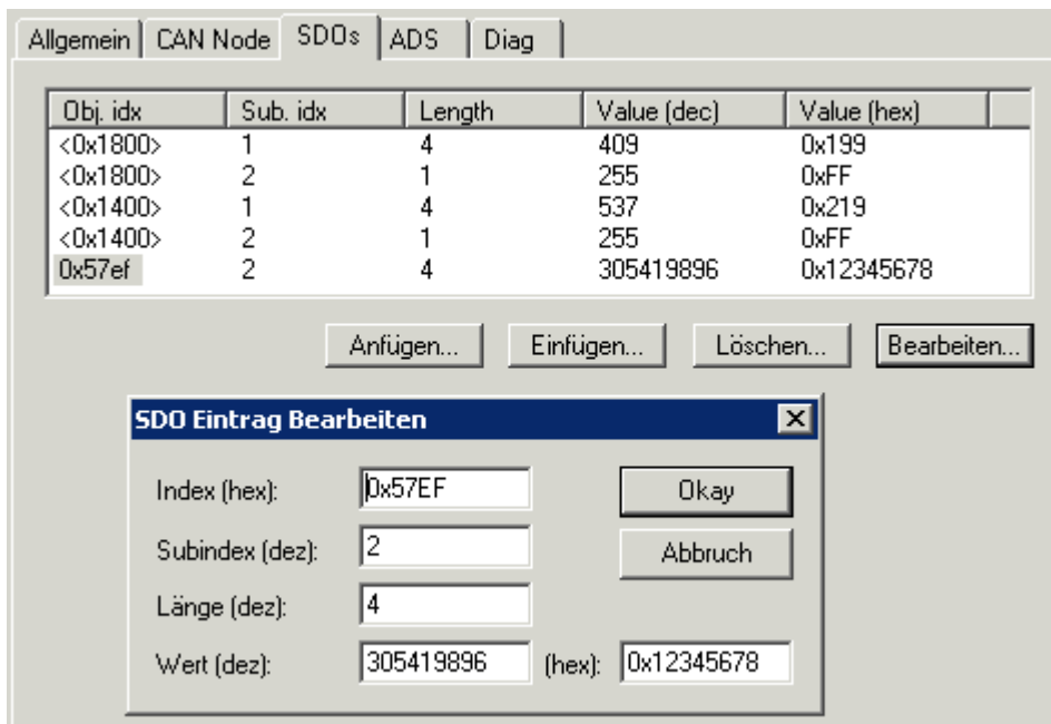
Fig. 57: Adding/editing object directory entries
