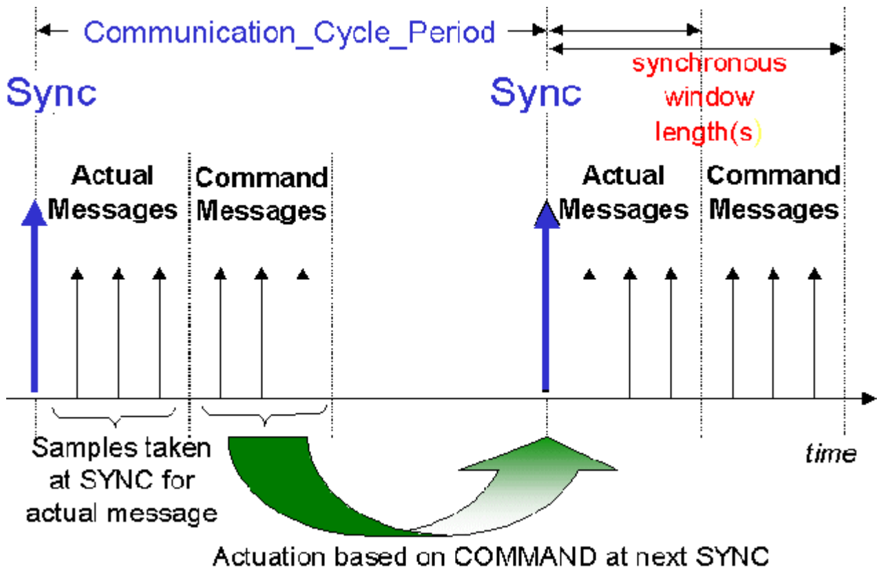
Fig. 134: Diagram: CAN "SYNC" telegram
