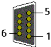
Fig. 16: COM1 (RS 232) and COM2 (RS 232/485) interface
