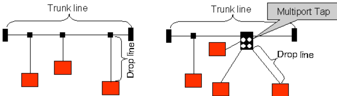
Fig. 19: Sample topology of drop lines
