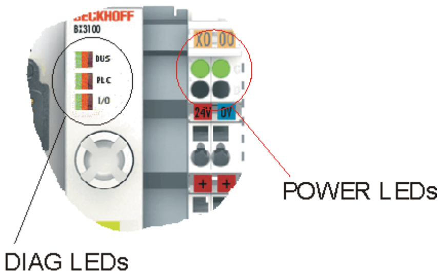
Fig. 143: Diagnostic LEDs for the fieldbus, the PLC, the K-bus and the power supply units
