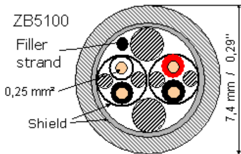
Fig. 20: Structure of CAN cable ZB5100
