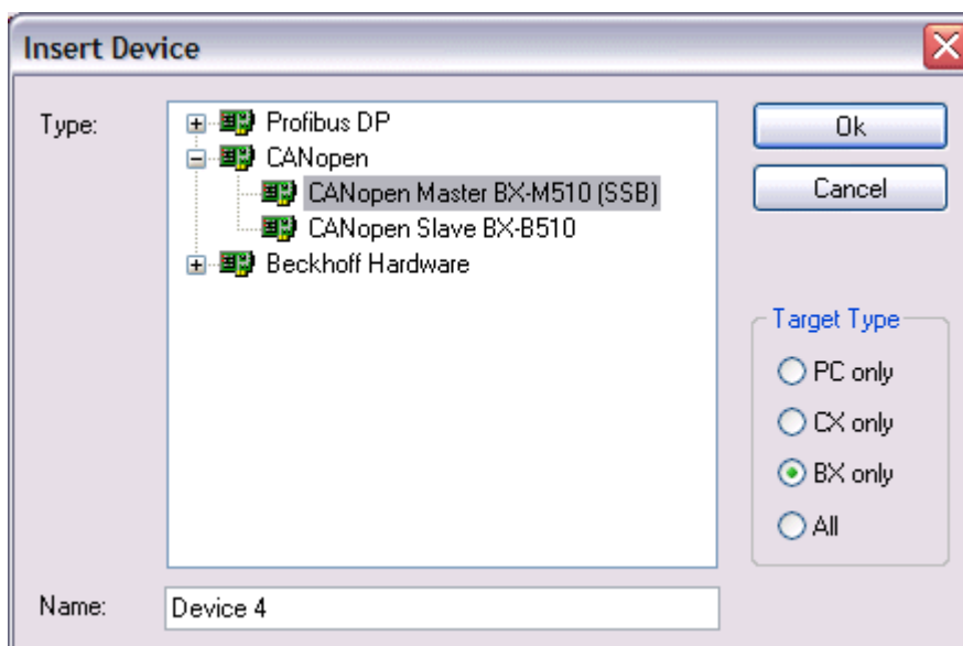
Fig. 54: Selecting the CANopen master SSB
