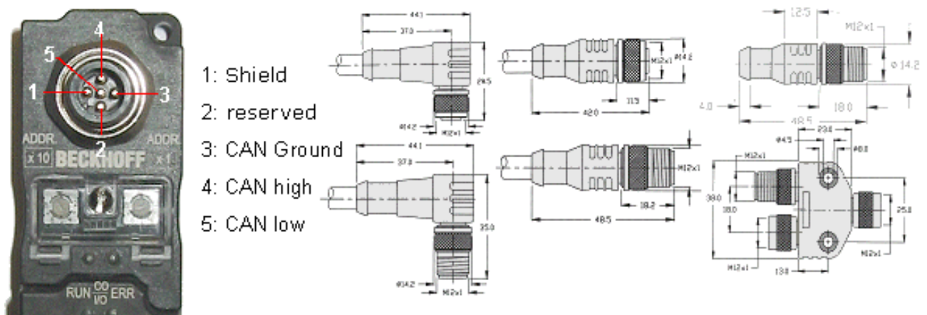
Fig. 26: Pin assignment: M12 plug, fieldbus box
