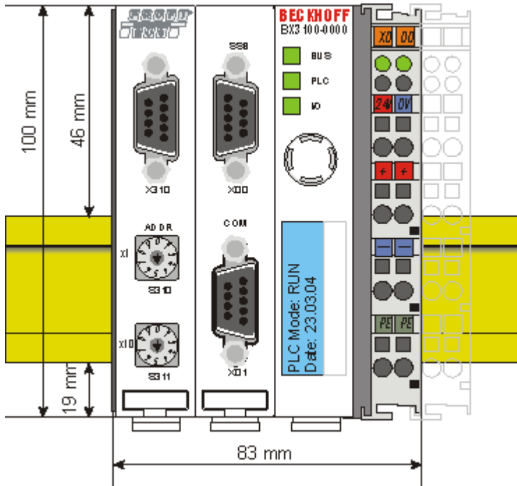
Fig. 3: BX3100, BX5100, BX5200, BX9000
