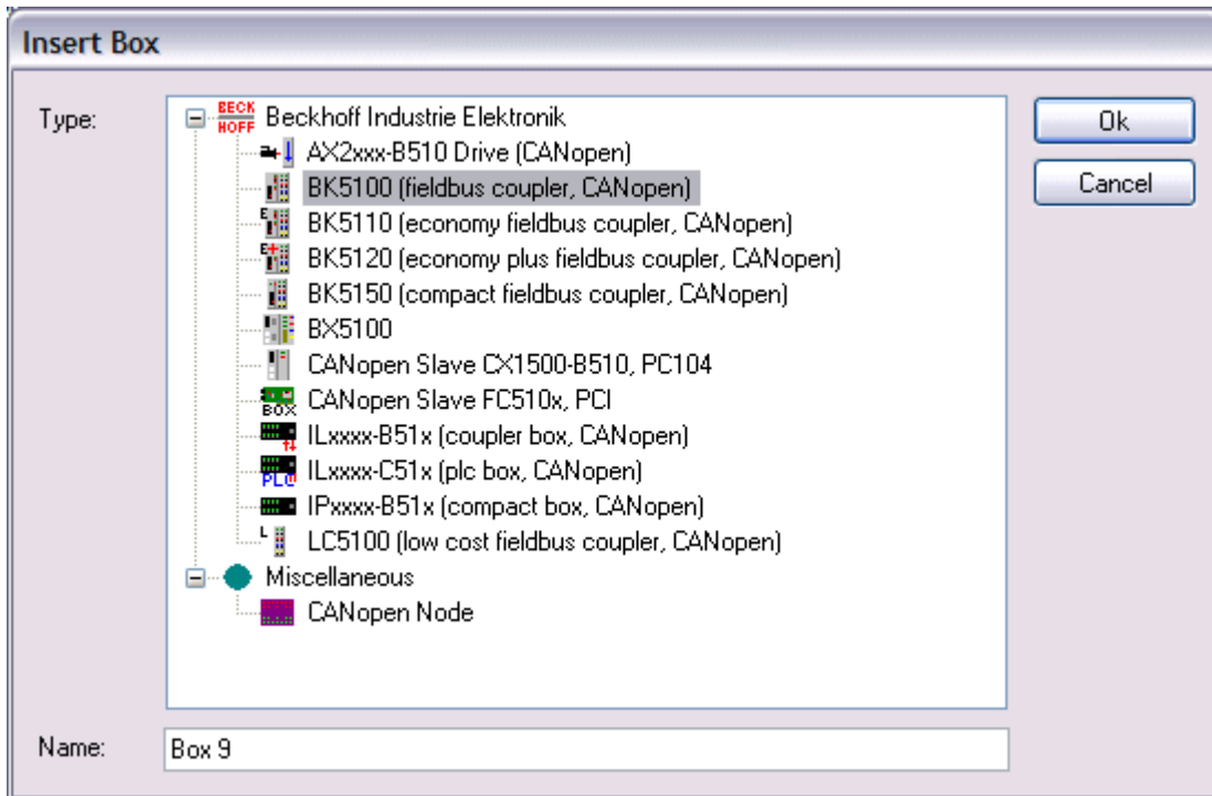
Fig. 56: Selecting a CANopen node
