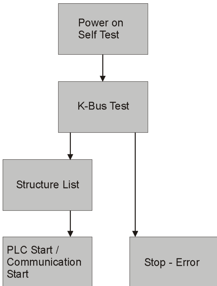
Fig. 27: Start-up behavior of the Bus Terminal Controller
