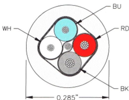
Fig. 21: Structure of CAN/DeviceNet cable ZB5200
