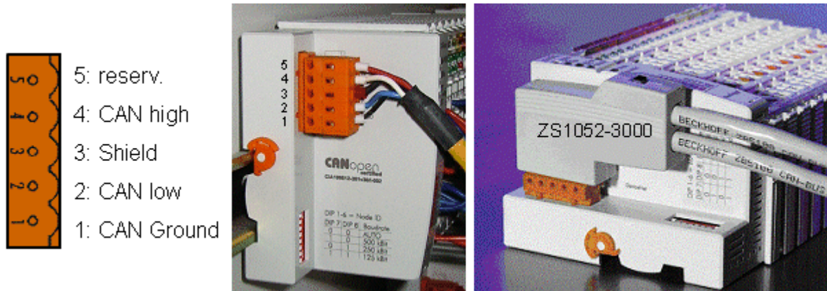
Fig. 24: BK51x0/BX5100 socket assignment
