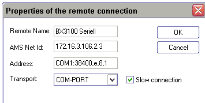
Fig. 42: Properties of the remote connection
