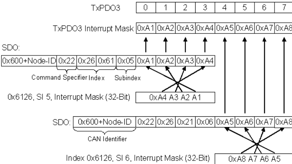
Fig. 140: Example for data assignment
