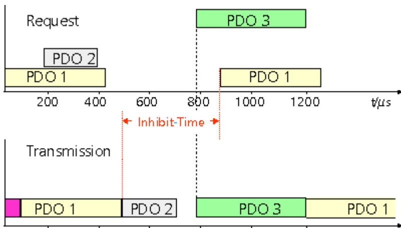
Fig. 43: Send delay time (inhibit time)
