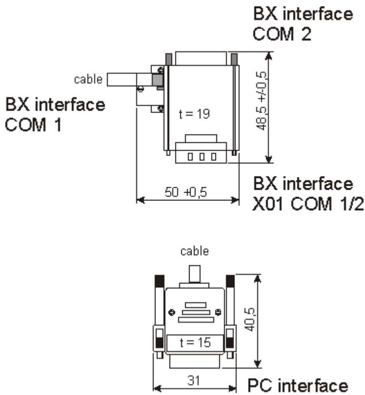
Fig. 13: Programming cable ZK1000-0030 - plug connector dimensions
