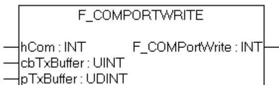
Fig. 92: Function block F_COMPORTRWRITE
