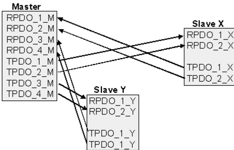
Fig. 131: Default identifier allocation: Master/Slave
