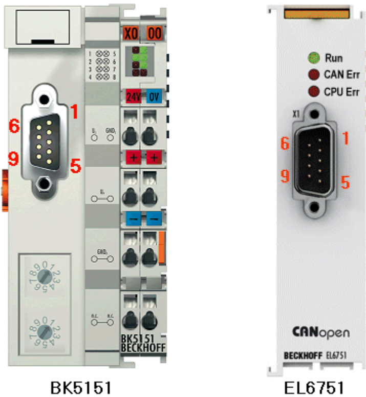
Fig. 22: BK5151, EL6751 pin assignment
