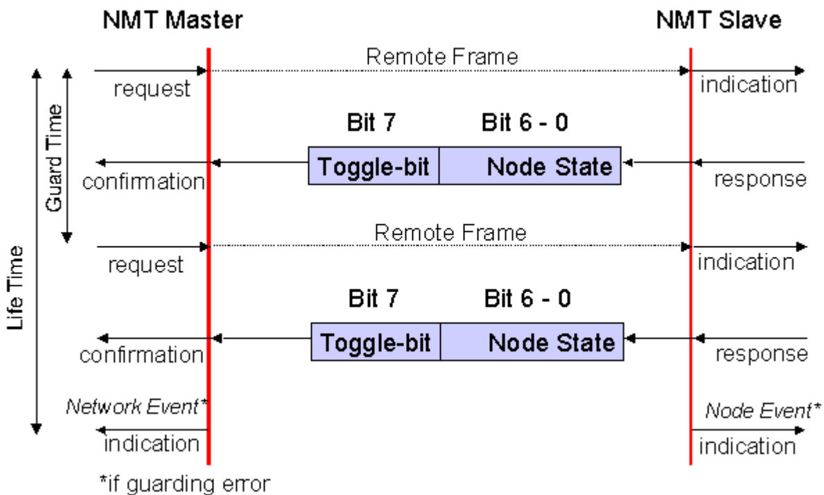
Fig. 129: Schematic diagram: "Guarding procedure"
