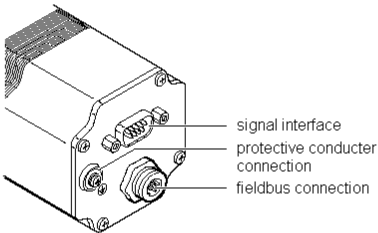
Fig. 64: IclA drive connections
