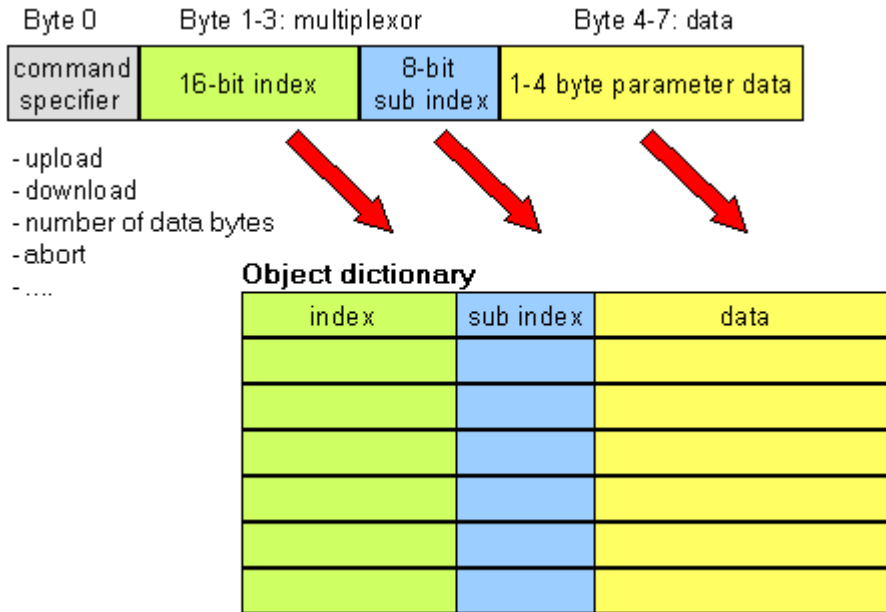
Fig. 138: SDO protocol: access to the object directory
