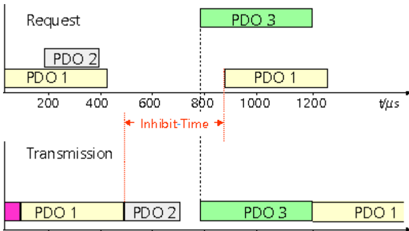
Fig. 135: Timing diagram: "Inhibit time"
