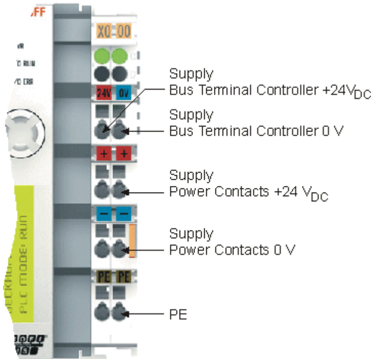
Fig. 10: Terminal points for the Bus Terminal Controller supply
