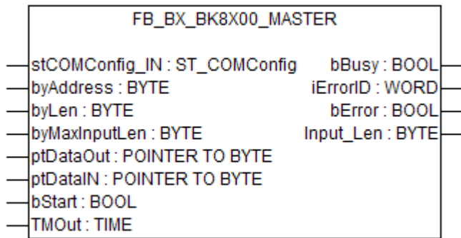
Fig. 101: Function block FB_BX_BK8X00_master
