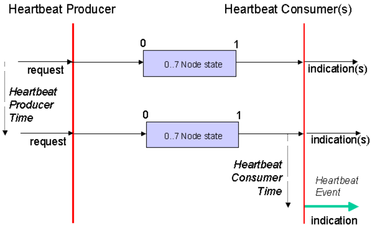
Fig. 130: Schematic diagram: "Heartbeat procedure"
