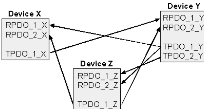
Fig. 132: PDO linking: Peer to Peer
