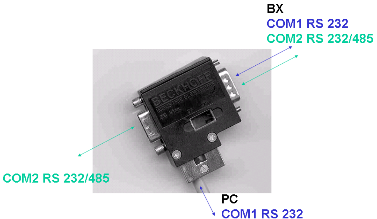
Fig. 12: Programming cable ZK1000-0030 - COM 1 and COM 2
