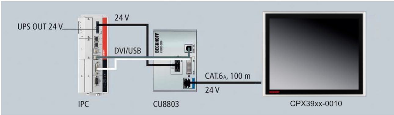
Fig. 5: CP-Link 4-One cable display Link via the CU8803 transmitter box
