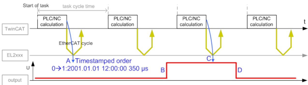
Fig. 17: Output of output channel information, with timestamp
