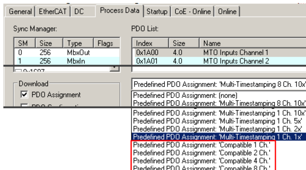
Fig. 160: Predefined PDOs for compatibility mode
