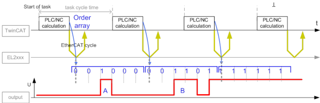
Fig. 16: Output of output channel information, oversampling
