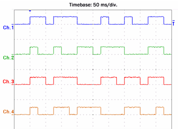
Fig. 173: Recording of four channels by the Multi-Timestamp program example
