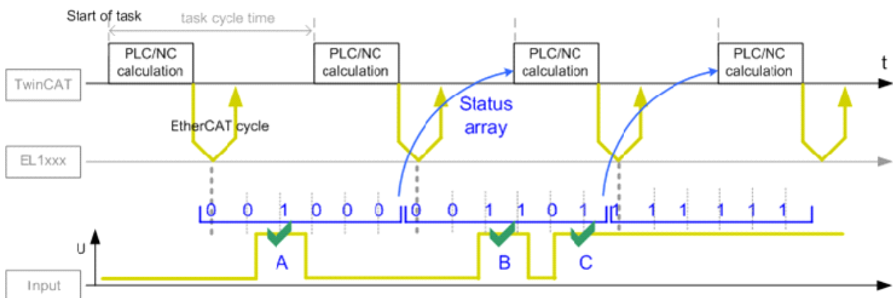
Fig. 13: Query of input channel information, oversampling
