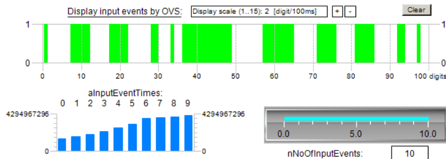
Fig. 177: Sample program EL1258 / Visualization_2: Display of incoming events in chronological order according to the timestamps of the EL1258
