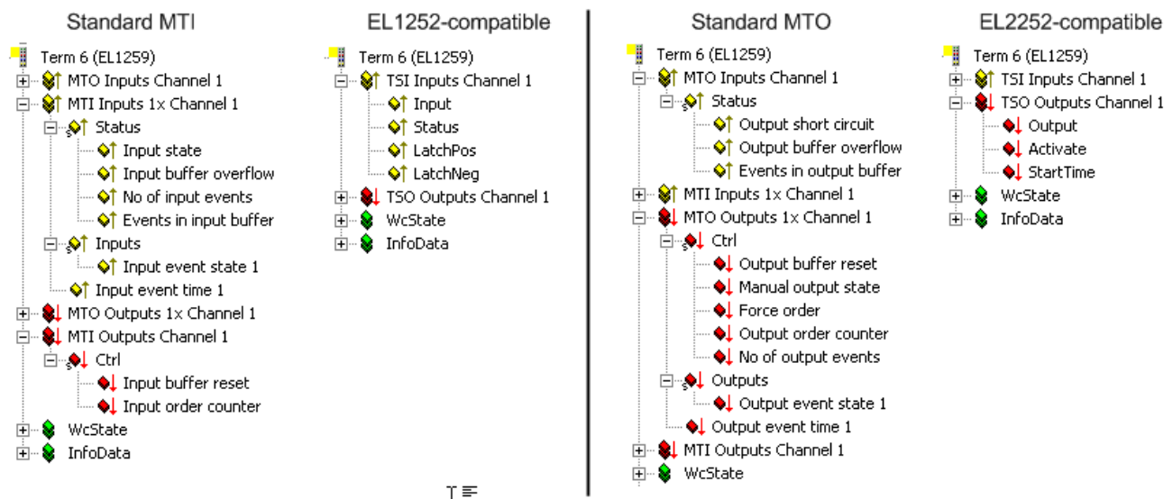
Fig. 148: Option for setting of compatibility modes in relation to EL1252/EL2252
