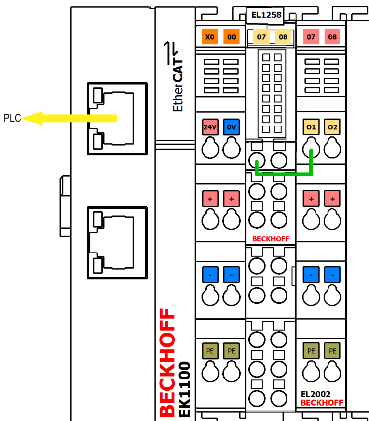
Fig. 174: Recommended structure for the EL1258 sample program
