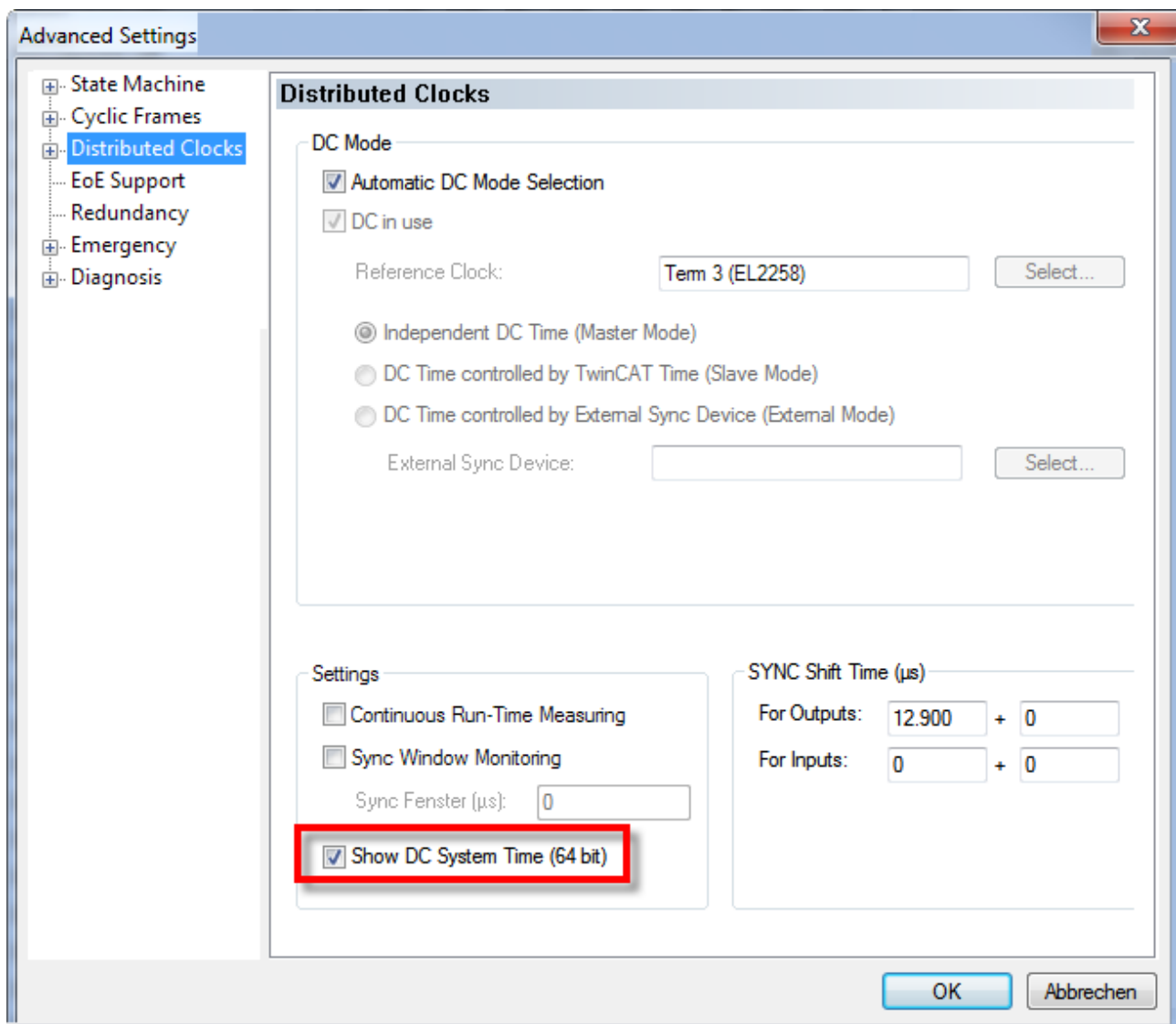
Fig. 168: Activation of the master distributed clock display
