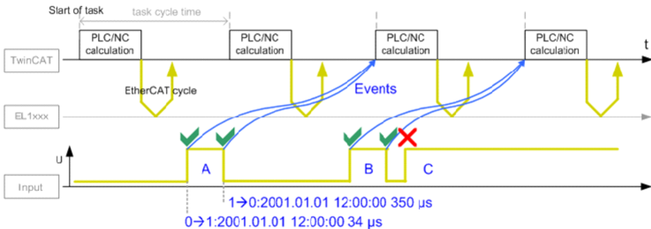
Fig. 14: Query of input channel information, with timestamp
