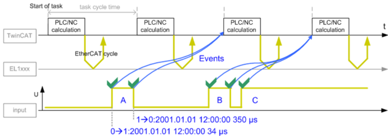
Fig. 18: Query of input channel information, with multi-timestamp
