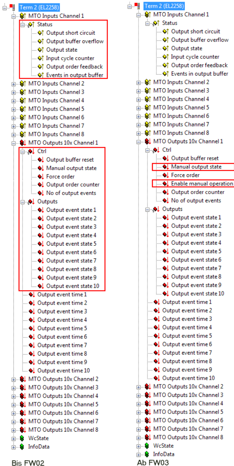
Fig. 161: Inputs and outputs in the project tree
