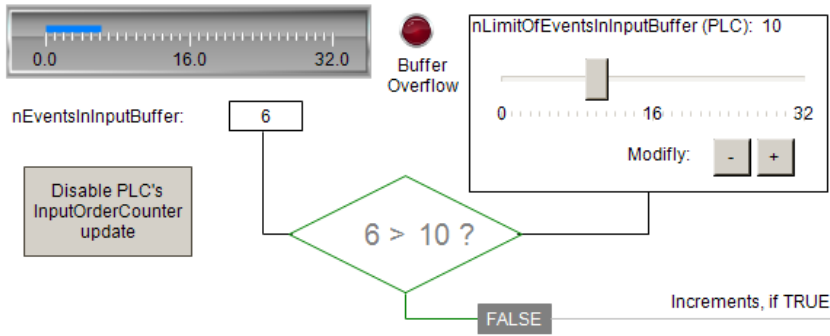
Fig. 178: Query of the "EventInInputBuffer" of the EL1258: Are there any other events stored in the terminal?
