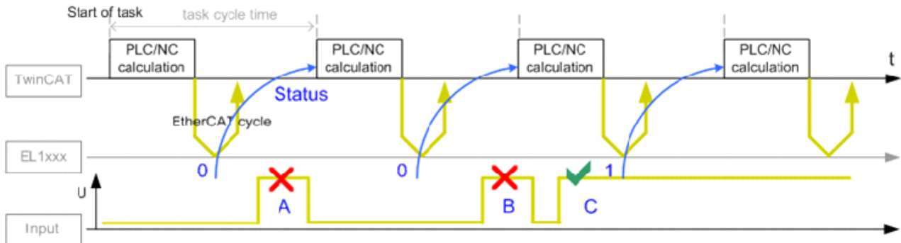
Fig. 12: Query of input channel information, standard
