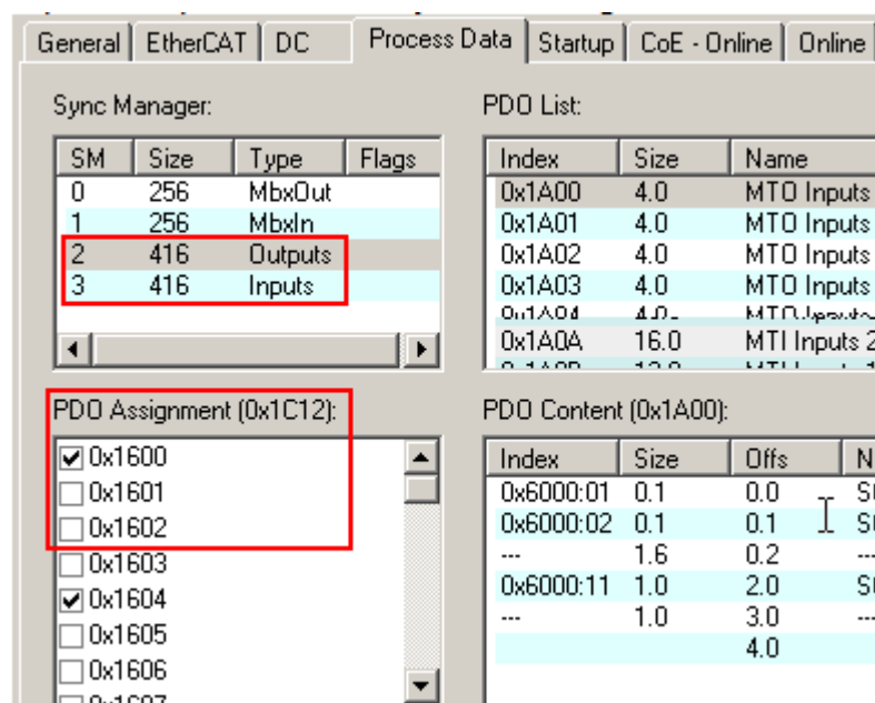
Fig. 150: Free selection of the PDO
