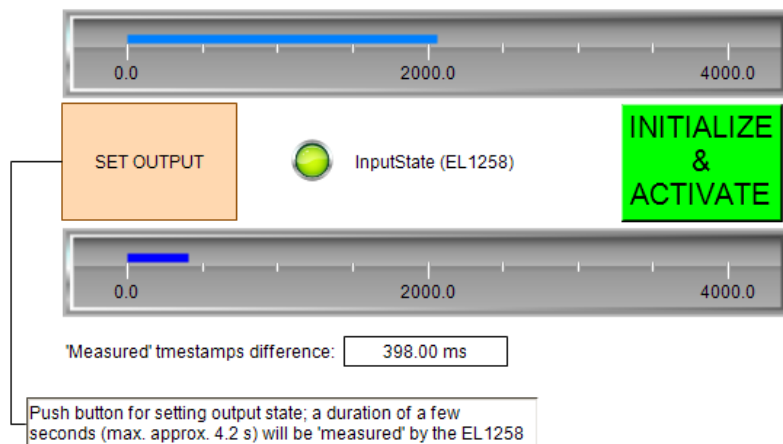
Fig. 176: Sample program EL1258 / Visualization_1: simple time measurement based on two state changes
