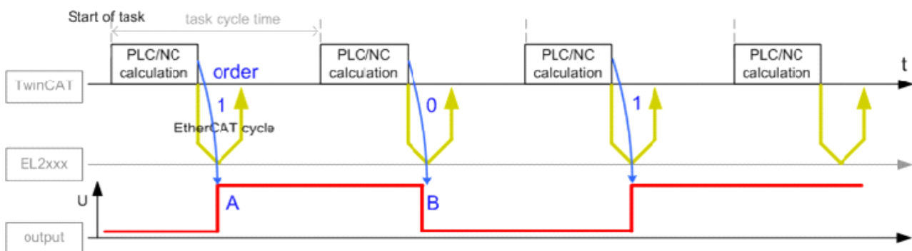
Fig. 15: Output of output channel information, standard
