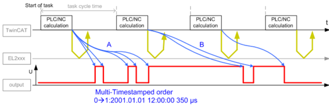
Fig. 19: Output of output channel information, with multi-timestamp
