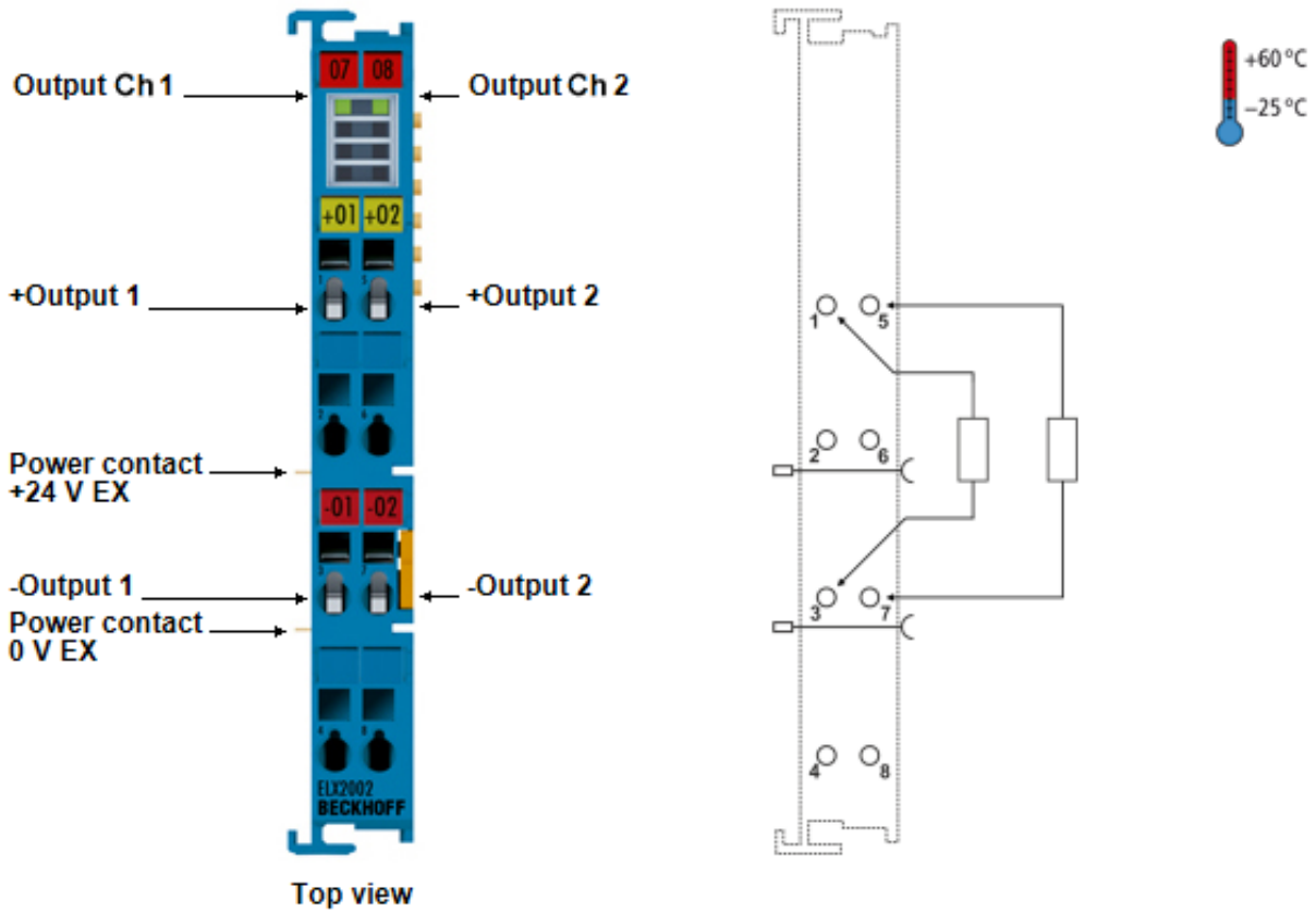
Fig. 3: ELX2002 - Two channel, digital output terminal, 24 V DC , 45 mA, Ex i
