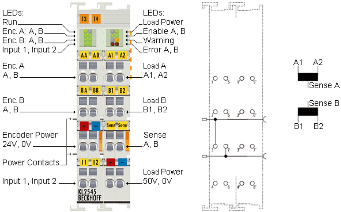
Fig. 20: KL2545 Connection
