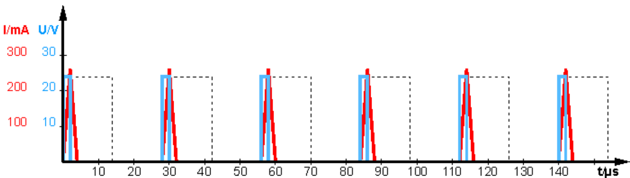
Fig. 6: Operation at load inadequate inductance (near ohmic)
