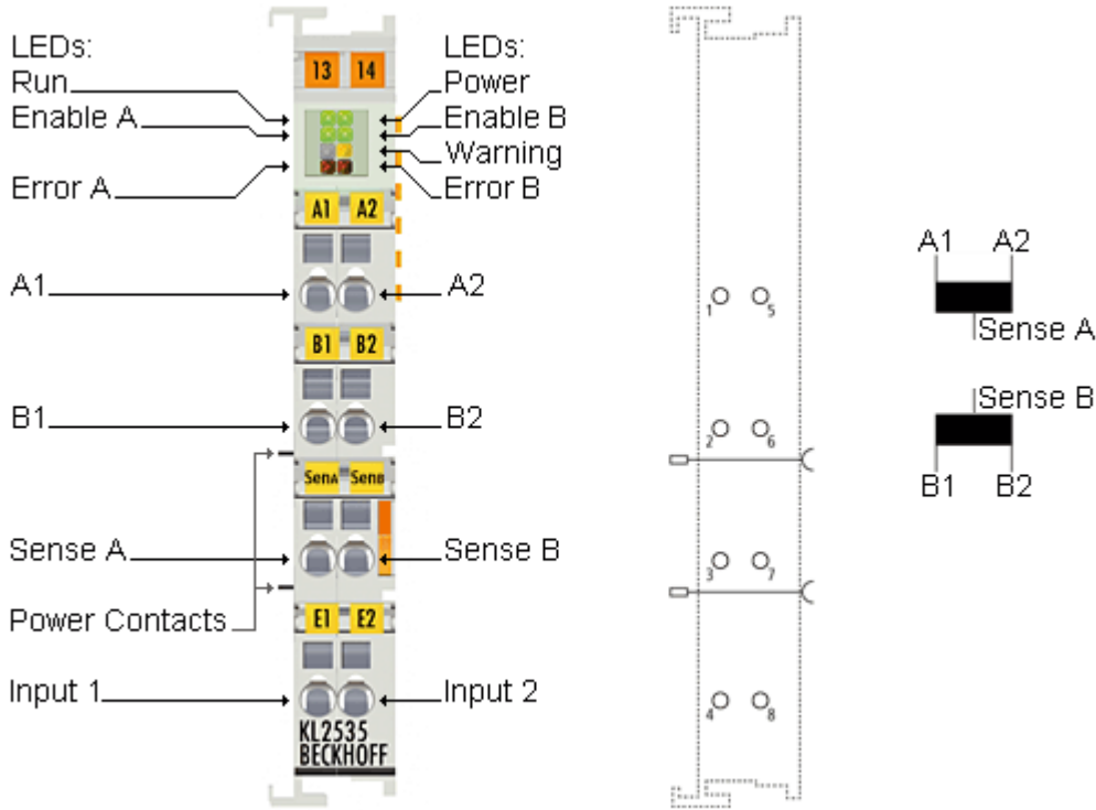
Fig. 19: KL2535 Connection
