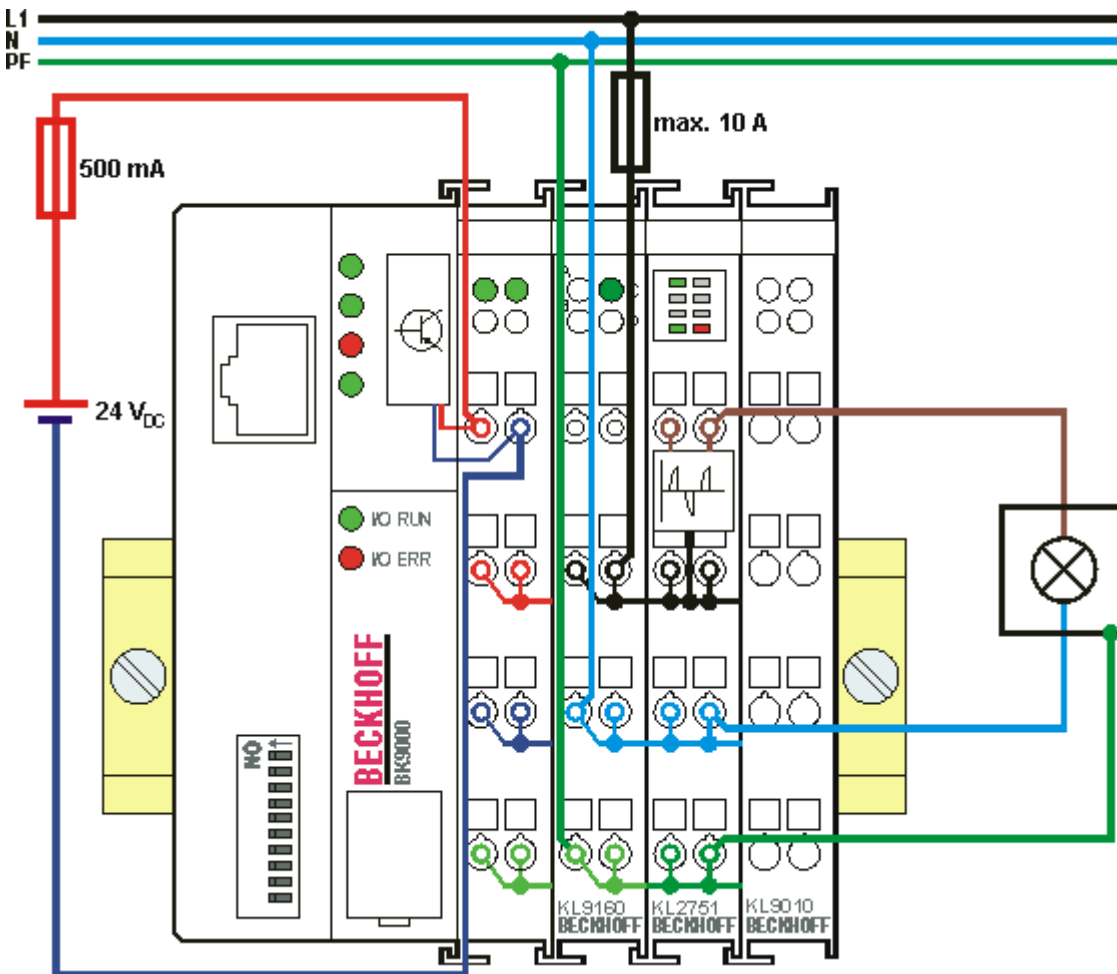
Fig. 15: KL2751-0000 connection example
