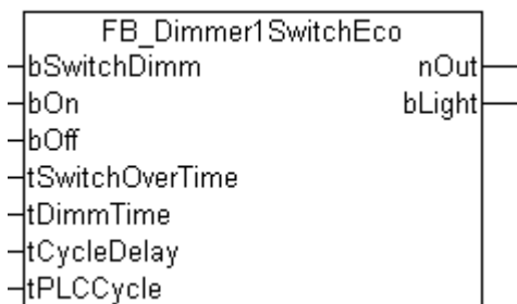
Fig. 27: FB_Dimmer1SwitchEco
