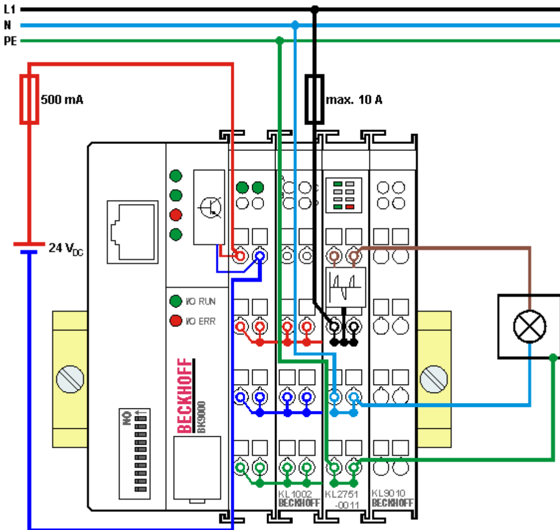
Fig. 16: KL2751-0011 - Application example
