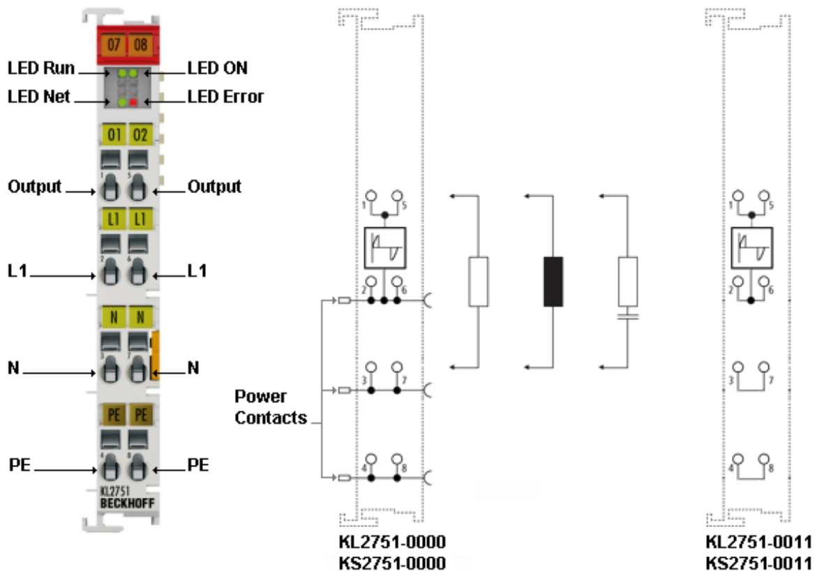
Fig. 14: Connection taking KL2751 as an example
