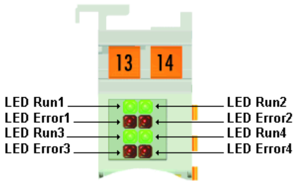
Fig. 3: KL3444, KL3454 - Diagnostic LEDs
