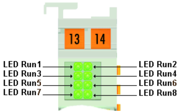
Fig. 6: KL3448 - Diagnostic LEDs
