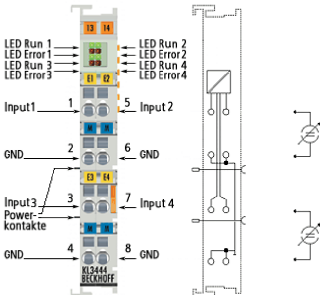
Fig. 17: KL3444 - Connection
