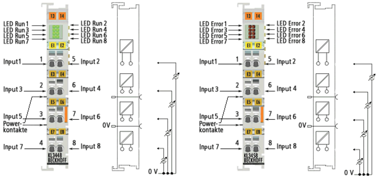
Fig. 19: KL3448, KL3458 - Connection
