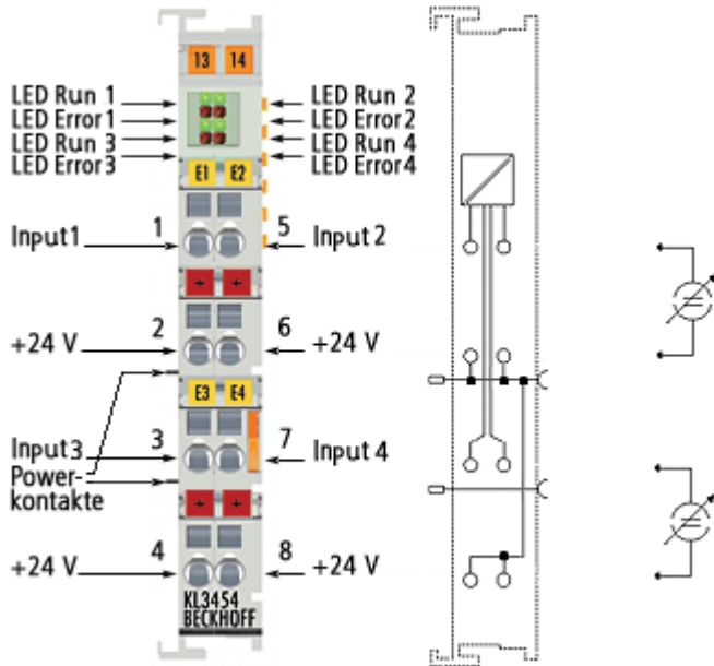
Fig. 18: KL3454 - Connection
