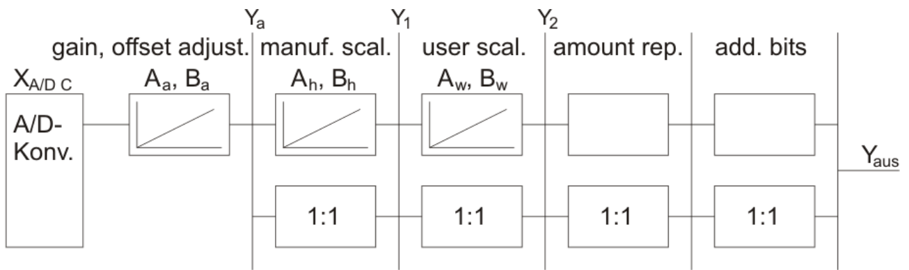
Fig. 8: Signal processing
