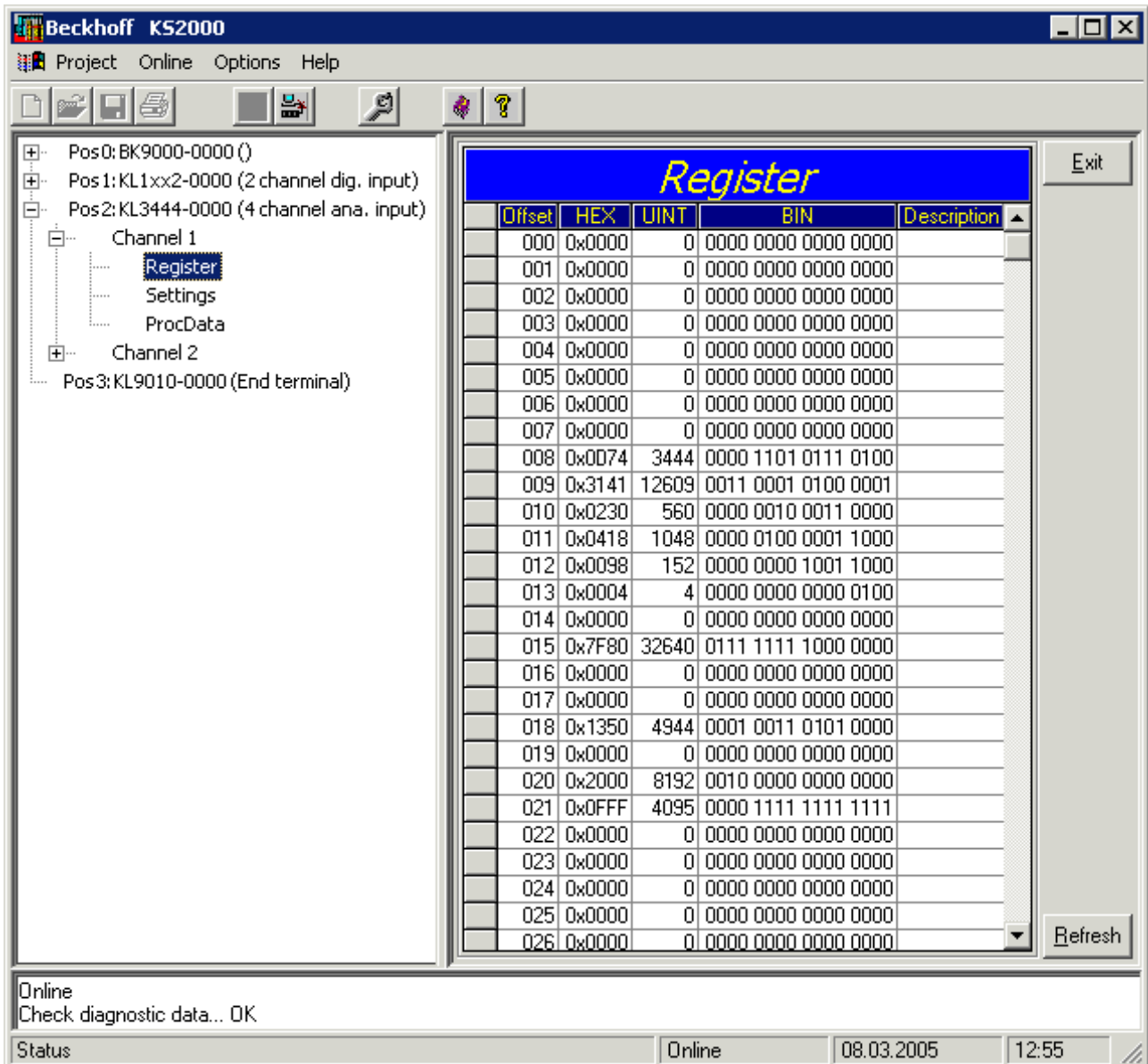
Fig. 24: Register view in KS2000
