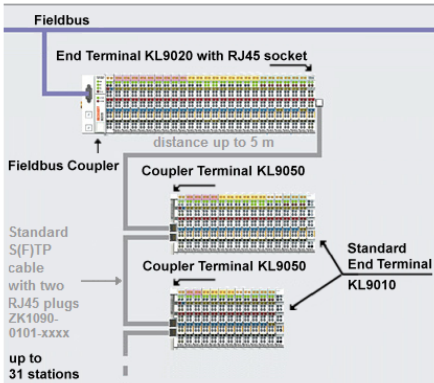
Fig. 1: KL9020 and KL9050 in the Beckhoff Bus Terminal system
