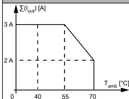
BWU2645, BWU2810, BWU3510 Derating total current of outputs
