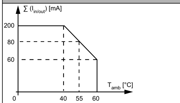
(2) BWU3577, BWU3695 Derating total current of inputs and outputs
