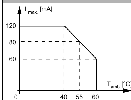
BWU3374, BWU3632, BWU3633 Derating power supply of attached sensors
