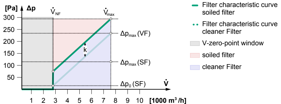
Fig. 85: Filter characteristic curve correction value
