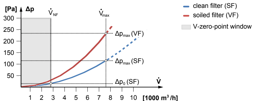
Fig. 83: Filter characteristic curve
