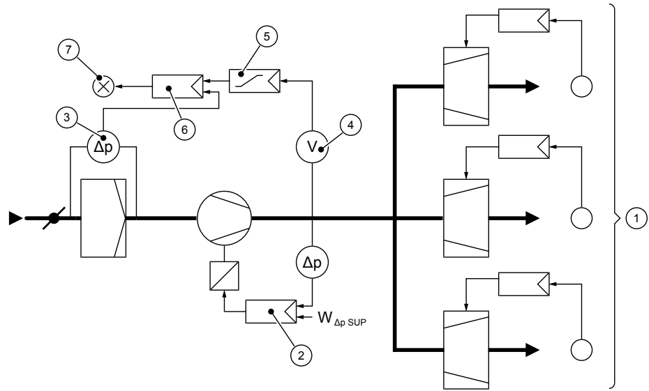
Fig. 81: Filter monitoring principle sketch
