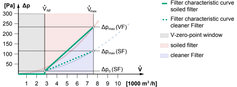
Fig. 84: Approximated filter characteristic curve
