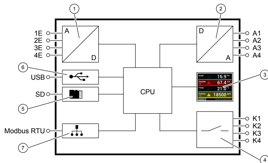
Fig. 1: Function diagram
