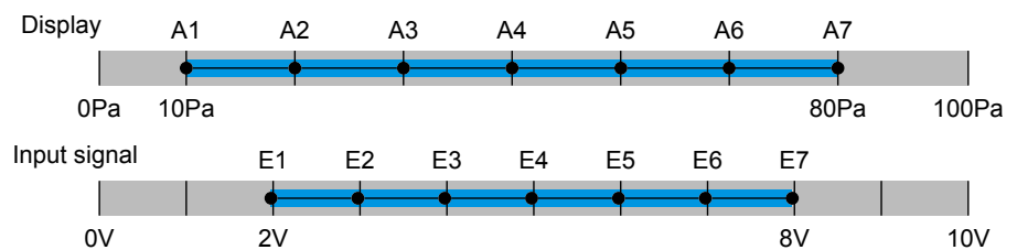
Fig. 74: Characteristic curve scale
