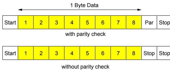
Fig. 101: MODBUS Bit Sequence
