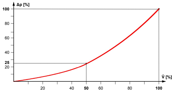
Fig. 82: Dependency on the volume flow
