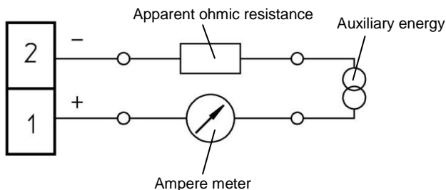
Fig. 3 Measuring switch
