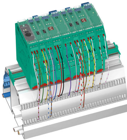
Profile rail with UPR-03- * insert, 3 conductors, wiring comb field side blue
