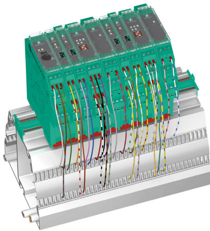
Profile rail with UPR-03-* insert, 3 conductors, wiring comb field side gray
