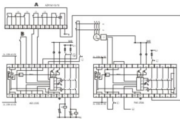
Wiring example
