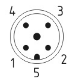
Contact arrangement
