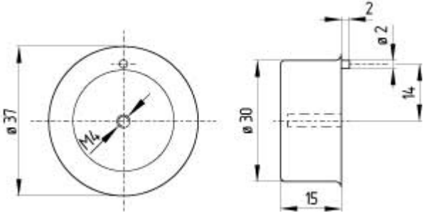
Dimensional drawing (miscellaneous)
