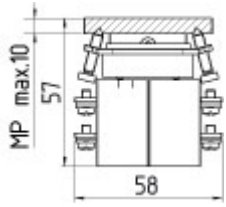
Dimensional drawing (miscellaneous)
