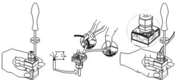
Assembly example
