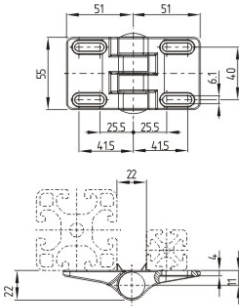
Dimensional drawing (basic component)
