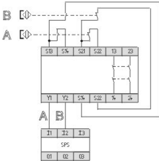
Wiring example
