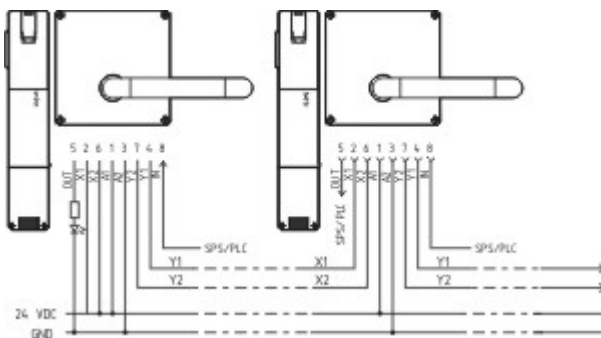
Wiring example
