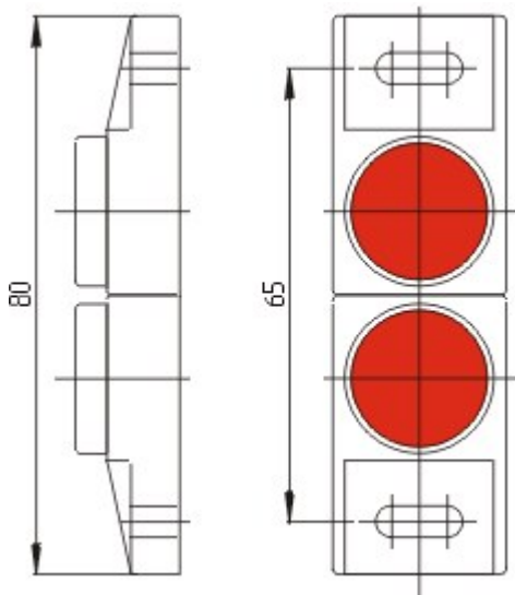
Dimensional drawing (miscellaneous)
