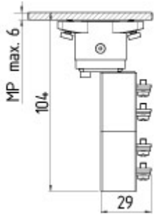
Dimensional drawing (miscellaneous)
