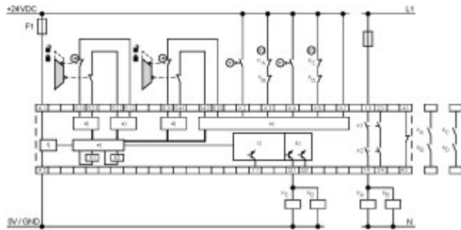
Wiring example
