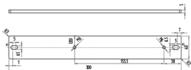
Dimensional drawing (miscellaneous)
