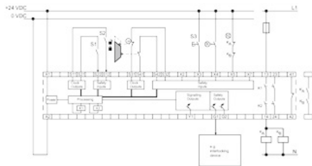
Wiring example
