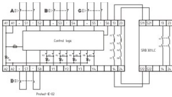
Wiring example
