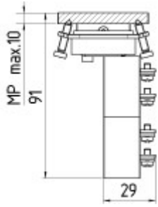
Dimensional drawing (miscellaneous)
