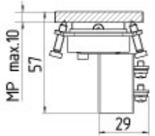
Dimensional drawing (miscellaneous)
