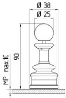
Dimensional drawing (miscellaneous)
