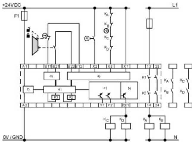
Wiring example
