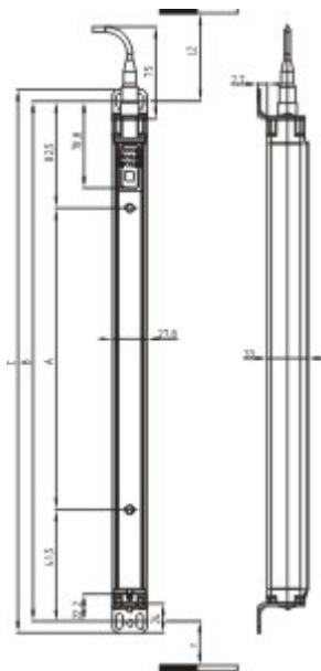
Dimensional drawing (basic component)
