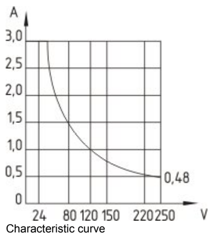
Characteristic curve
