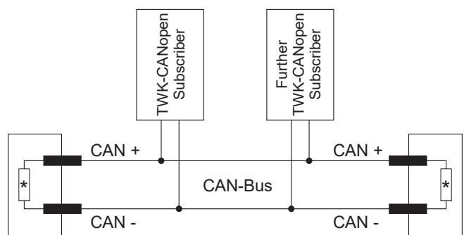
* Terminating resistor (120 Ω)
